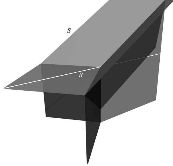
The rigid curve R in S .
