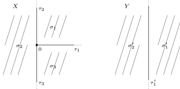
Fans X and Y such that \{\sigma \cap \sigma' \mid \sigma \in X, \sigma' \in Y\} is not a fan.
