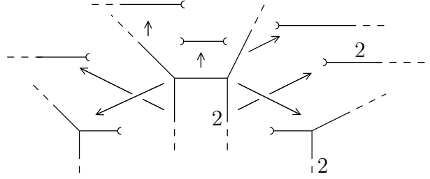
Figure 1.2: A weighted polyhedral complex together with the maps \Phi_\sigma .
